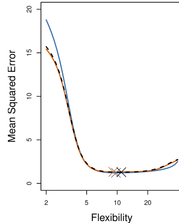
f(x) is highly nonlinear
