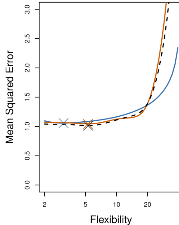
f(x) is close to linear
