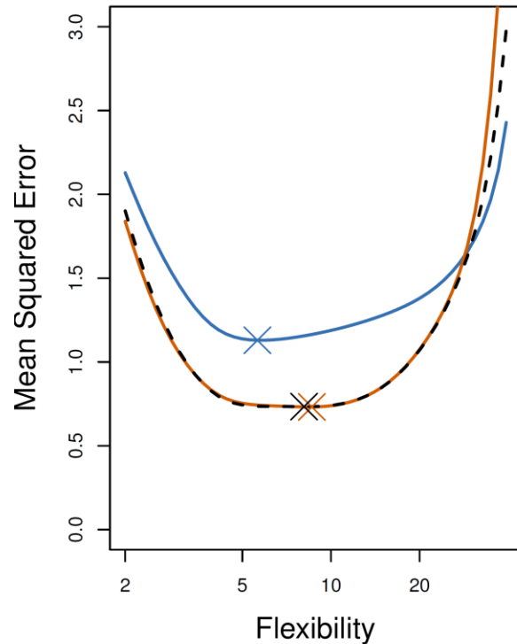
f(x) is a low order polynomial
